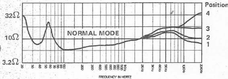
FIGURE 4 — Impedance vs Frequency
