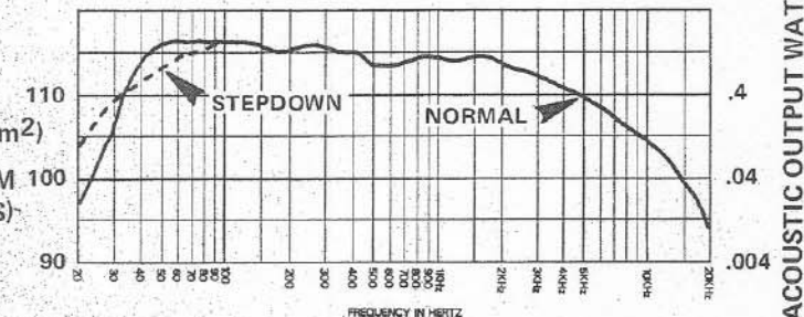
FIGURE 5 — Maximum Acoustic Output
